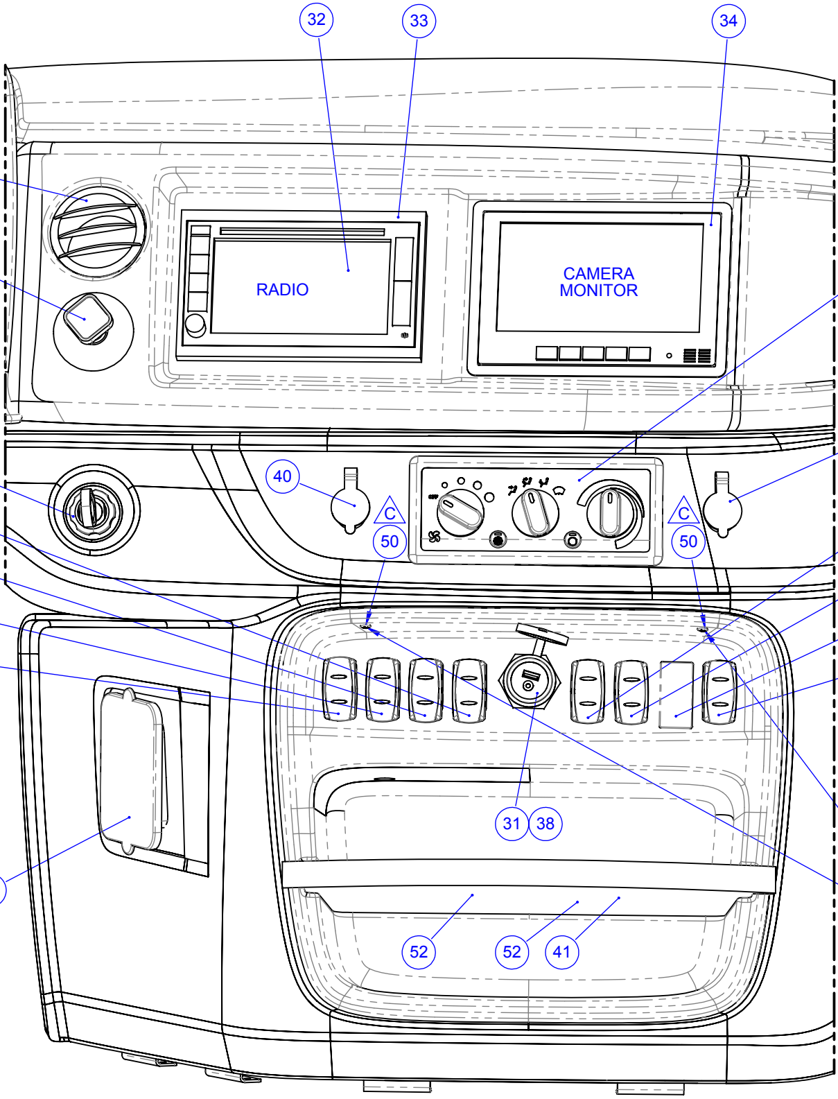
VIEW C
