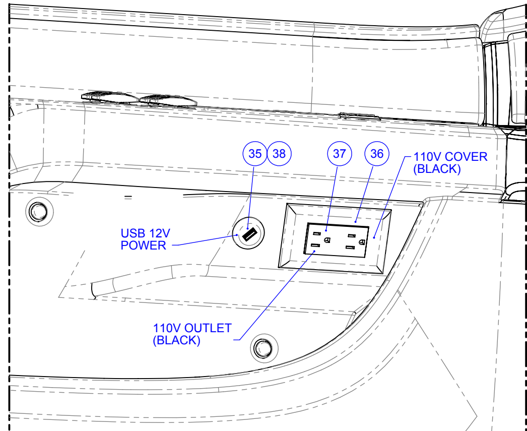
VIEW D
